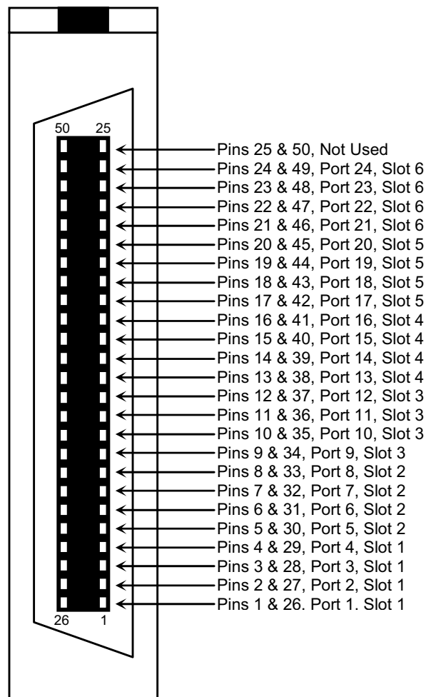
Figure A-1: RJ-21 Port Connector
